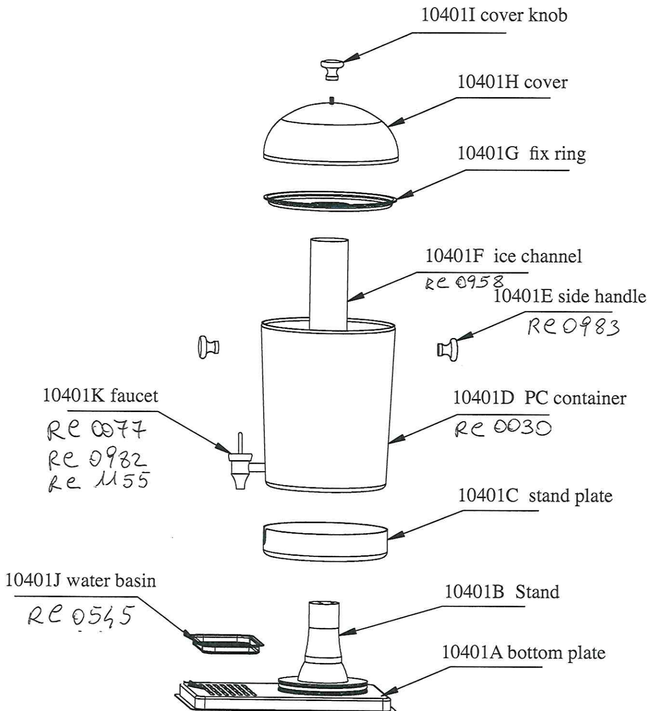
10401-2 Exploded drawing for juice
