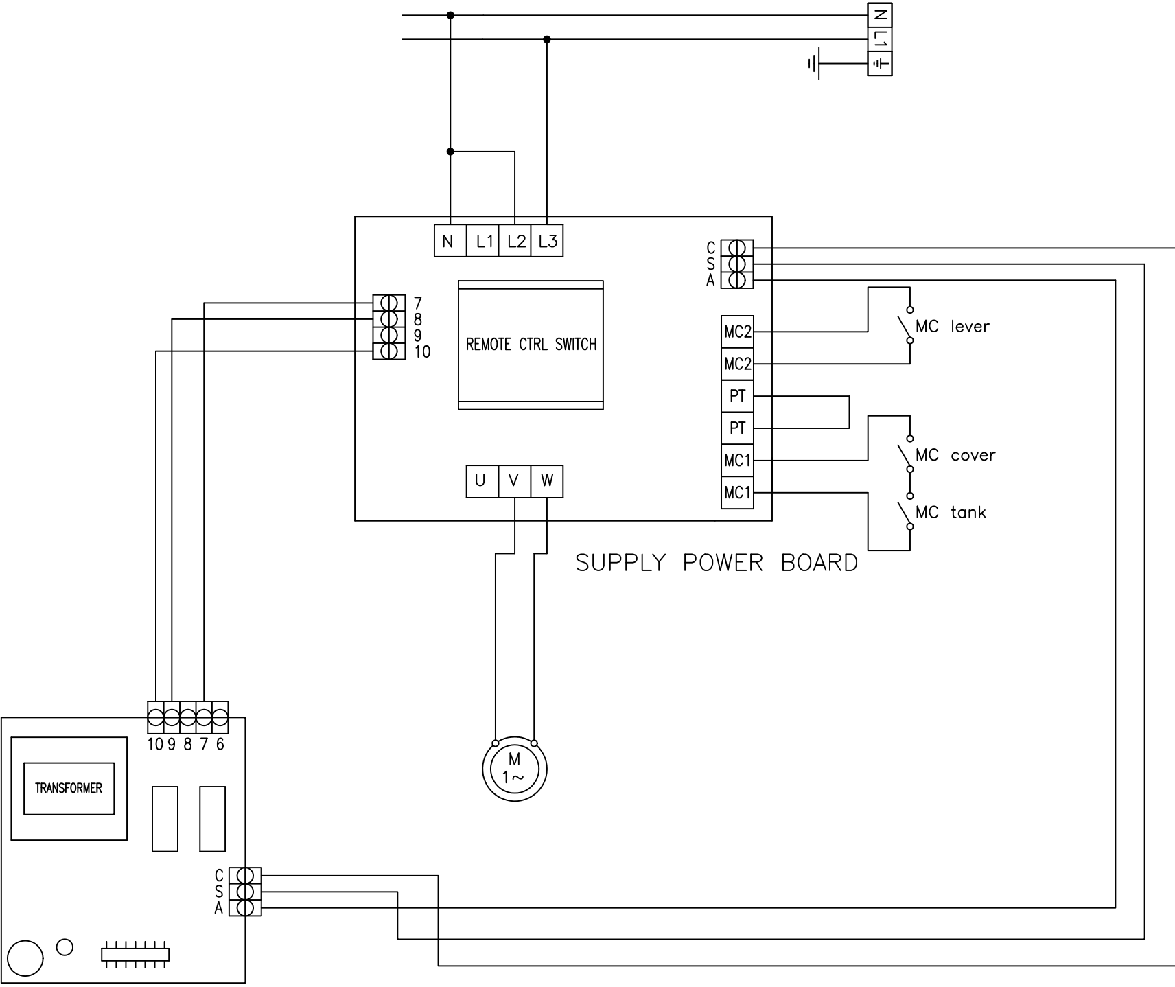
PUSH-BUTTON CONTROL BOARD
