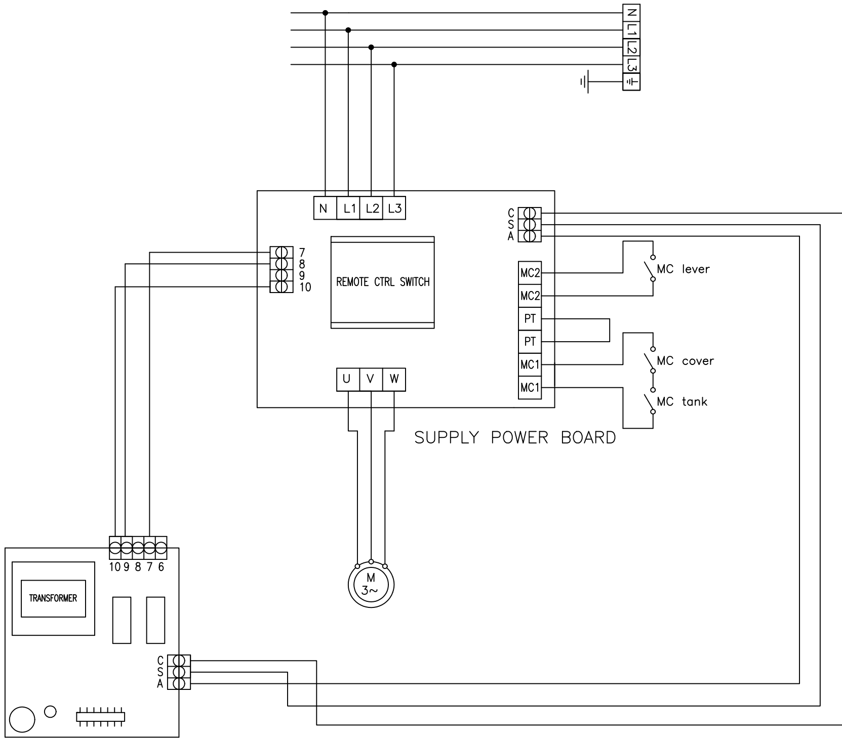
PUSH-BUTTON CONTROL BOARD
